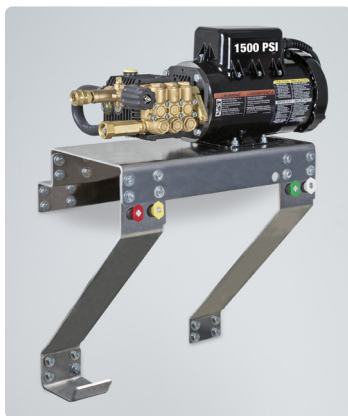
DC-1502-A0E1G-W (Stationary) shown with wall mount kit option, CX-0104
